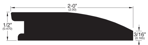
Reducer 010
