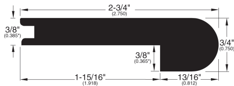
Stair Nose 009
