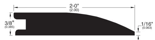
Reducer 007
