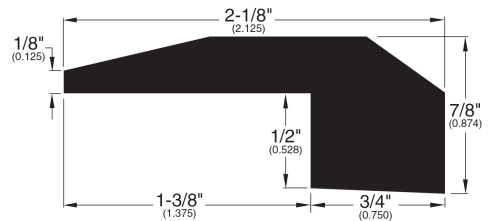
Threshold 011
