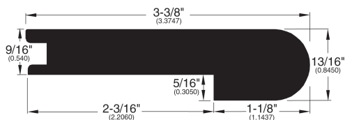
Stair Nose 021
