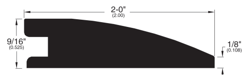
Reducer 020
