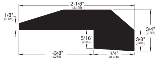
Threshold 008
