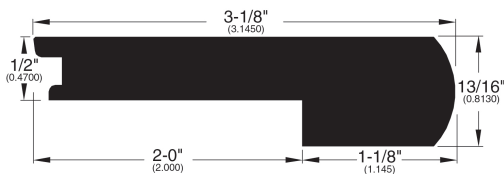
Stair Nose 012
