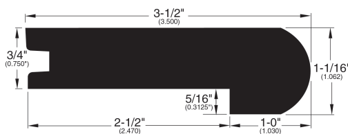
Stair Nose 061
